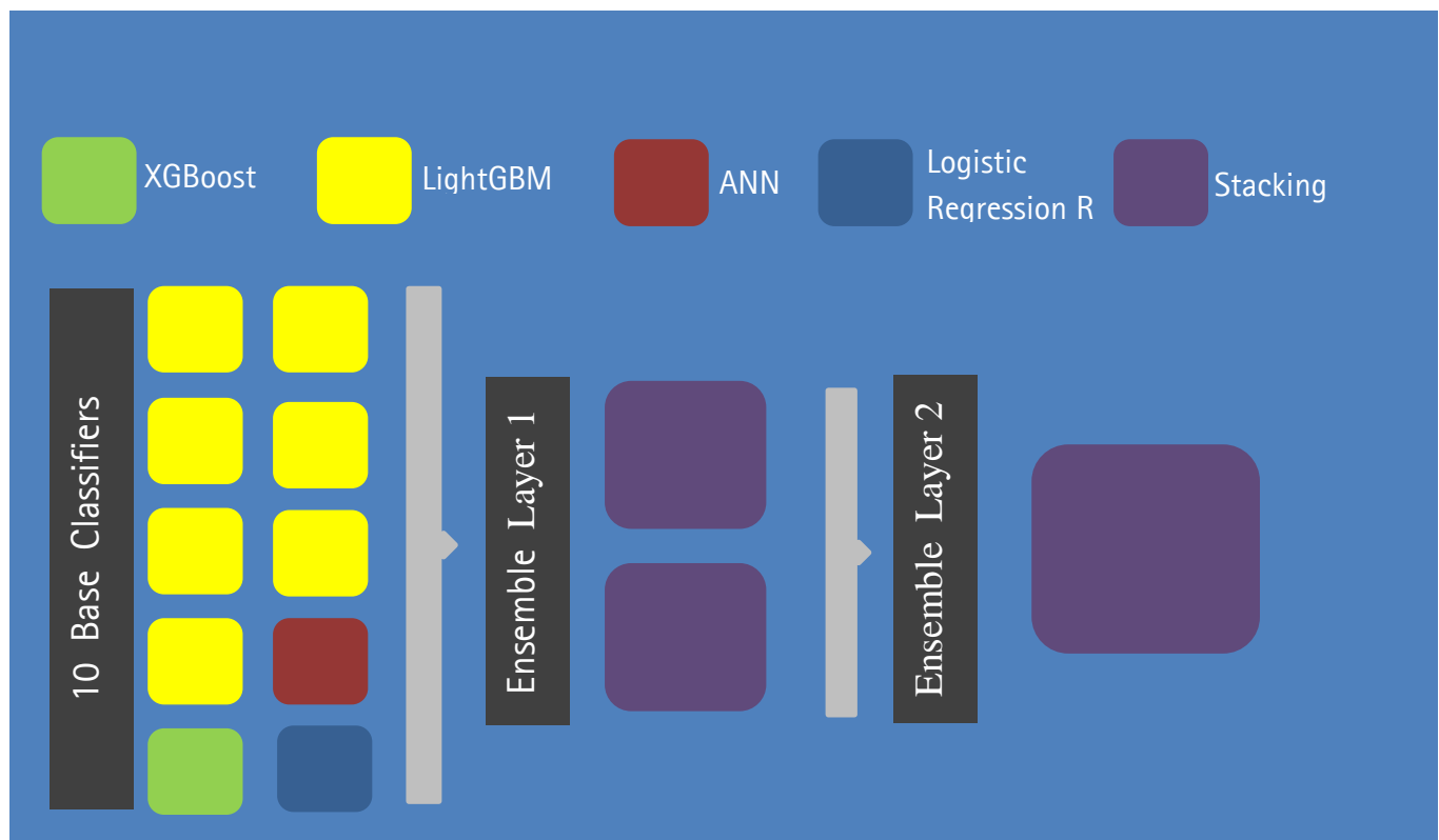
Figure 7 Modelling Architecture
